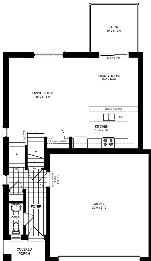
MAIN FLOOR
