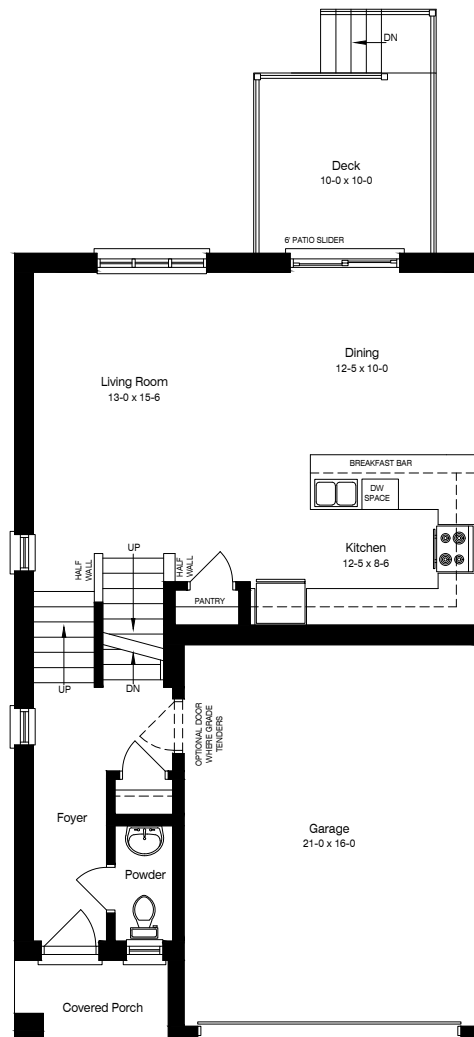
MAIN FLOOR
